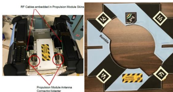
Fig. 5: REALM's Guest Science Payload. On the left, the integrated payload with Astrobee. On the right, REALM's customized Astrobee skin-antenna.
