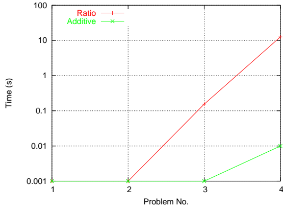
Figure 3: Additive versus ratio heuristic
