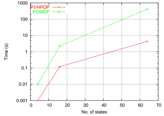
Figure 5: POMDP vs PVHPOP (threshold)
