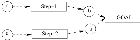
Figure 2: A partial plan
