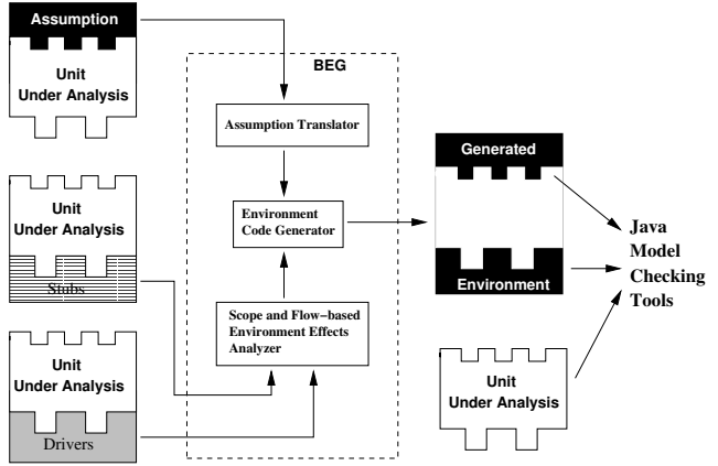
Figure 1. BEG Architecture
