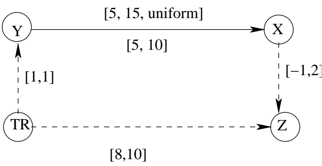
Figure 1: Example for calculating the upper bound.
