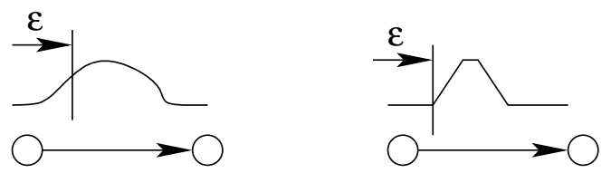
Figure 2: Two uncontrollable events with different distributions.
