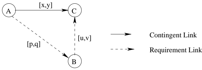
Figure 3: Triangular Networks (Morris, Muscettola, & Vidal 2001).
