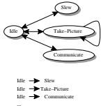
Figure 4: A simple state machine representation of the satellite domain. The rules implied by the state machine appear below the figure.
