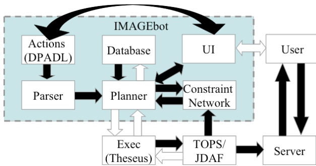
Figure 2: The agent architecture
