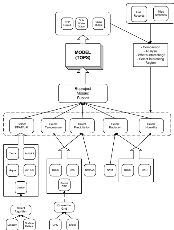
Figure 1: Data flow in the TOPS framework
