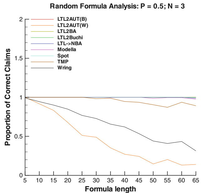
Fig. 9 Correctness degradation
