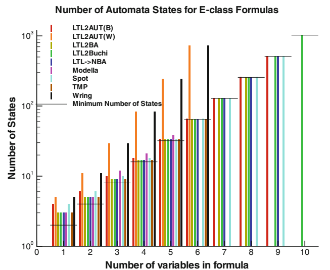
Fig. 8 E -Class formula data
