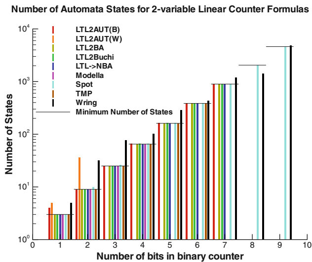
Fig. 11 Automata size: 2-variable linear counters
