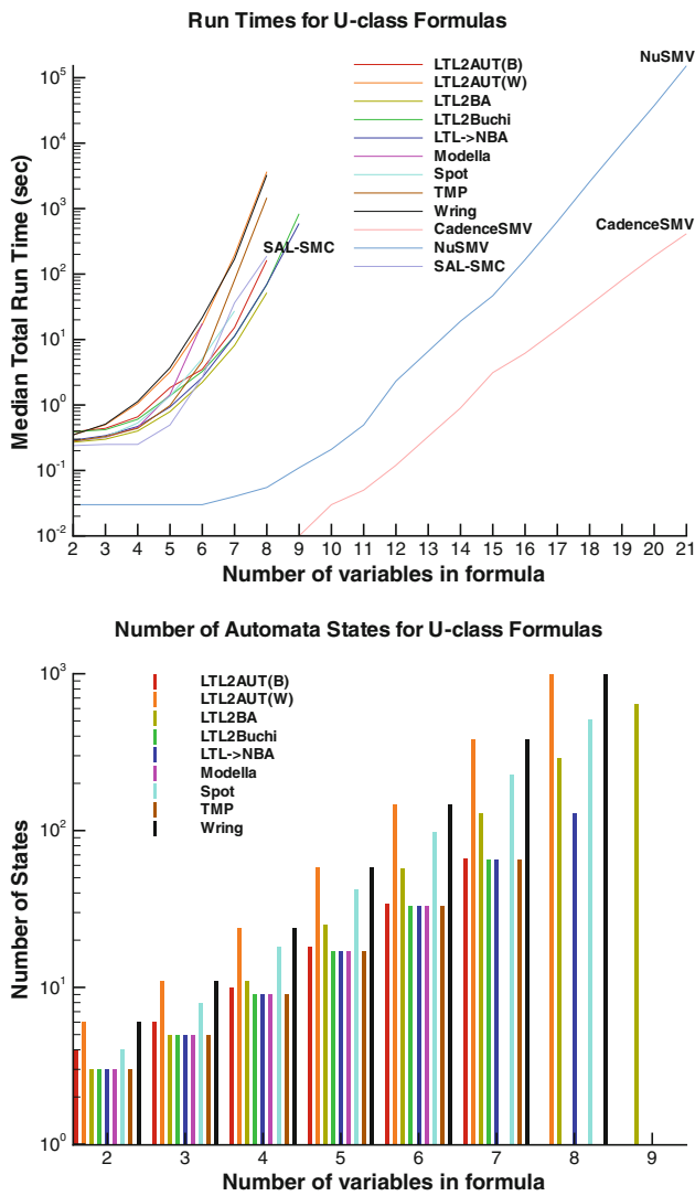
Fig. 13 U-Class formula data
