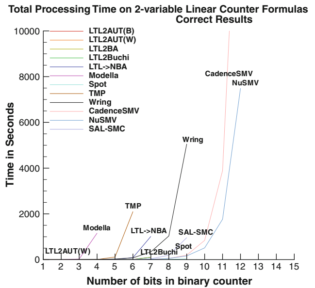
Fig. 4 Performance results: 2-variable linear counters
