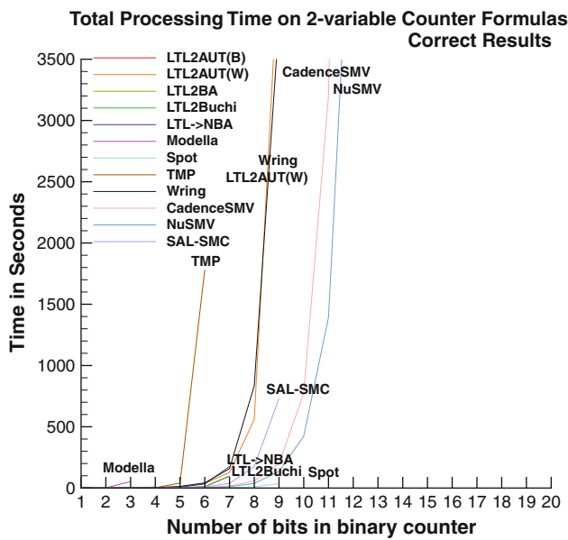
Fig. 3 Performance results: 2-variable counters
